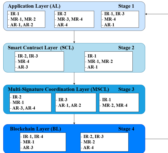
Figure 2: Mapping requirements to functionality layers
