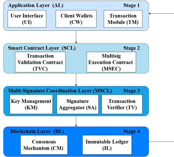
Figure 1: Layered Blockchain-based multisig
