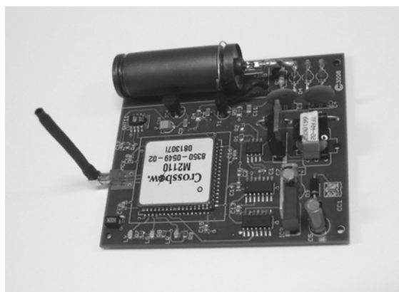
Figure 3. Prototype module integrating simple radiation sensor
