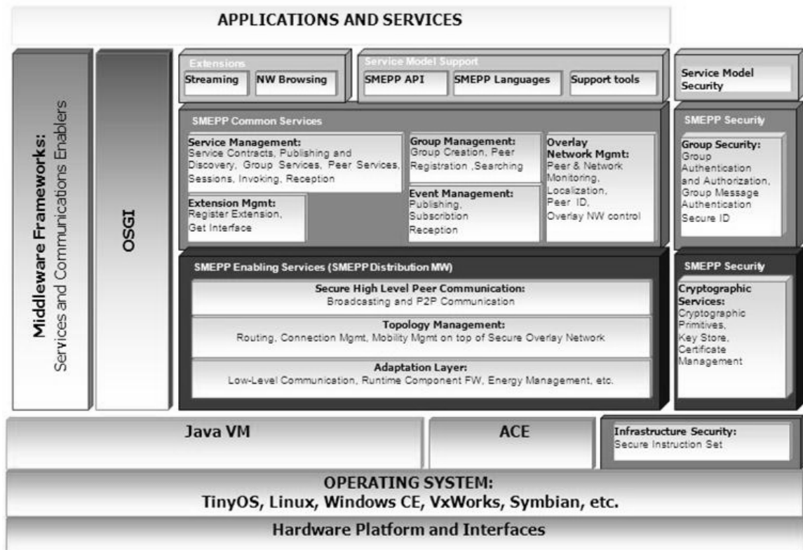
Figure 1: SMEPP Middleware Architecture in context
