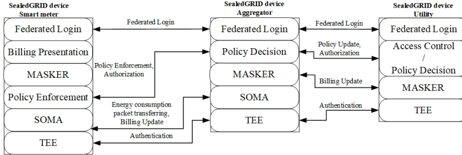
Figure 1: Architectural components and integrated modules for SealedGRID
